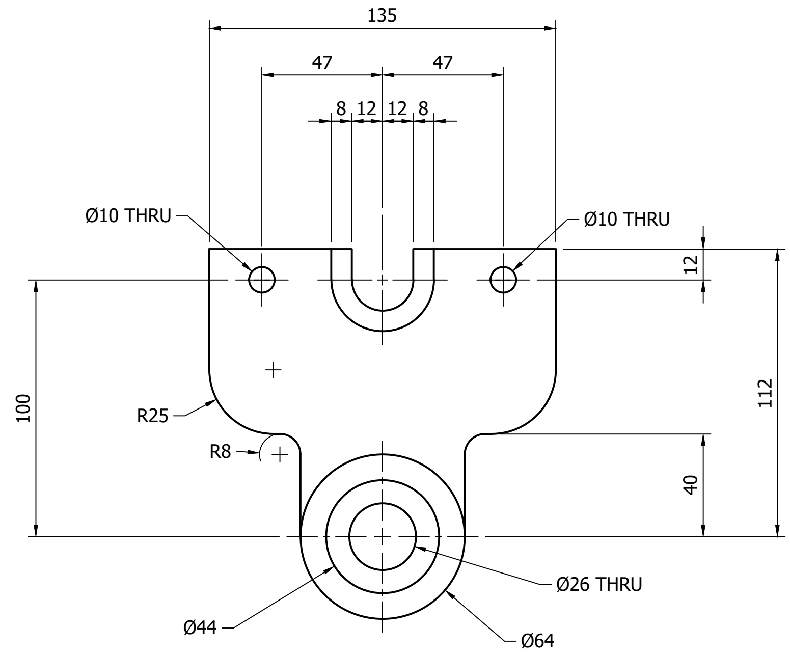
PIVOT BEARING
